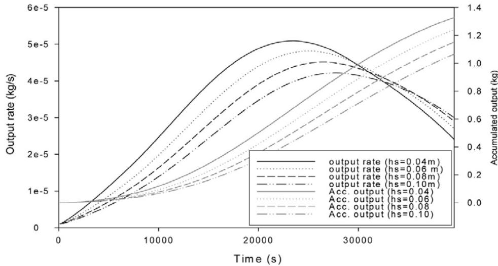
Fig. 4. System output at different depths of water with time.
