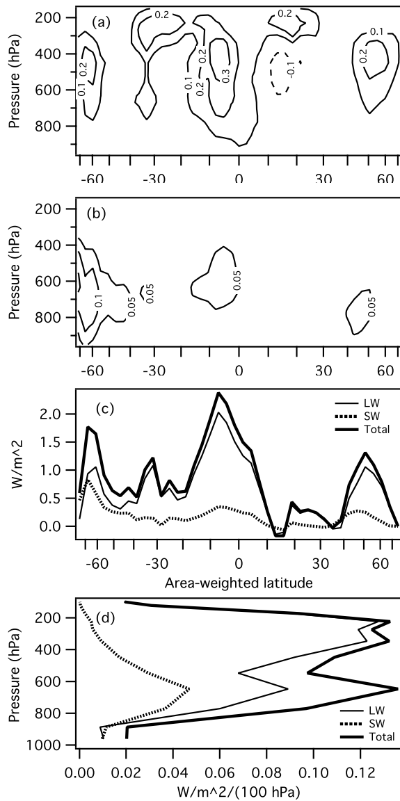
Figure 4. (a) Plot of LW component of (\partial R/\partial q)\Delta q ( W/m^2/(100 \text{ hPa}) ) due to the change in q between the January 2003–2007 average and January 2008, (b) same as Figure 4a, but for the SW component, (c) integral over pressure of the data in Figures 4a and 4b, with units of W/m^2 , (d) integral over latitude of the data in Figures 4a and 4b, with units of W/m^2/(100 \text{ hPa}) . In Figures 4a and 4b, solid contours indicate positive values and dashed contours indicate negative contours.
